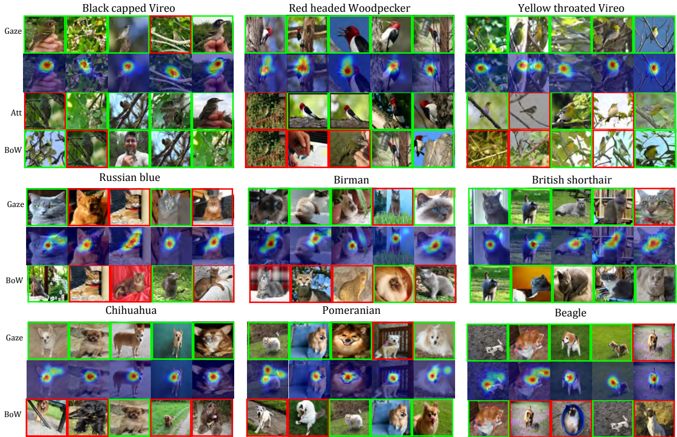
Figure 7: Qualitative Results: Five highest ranked images for unseen classes of birds, cats and dogs. We compare gaze with attributes (when available) and with bag of word representations and show gaze heat-maps of selected images.
